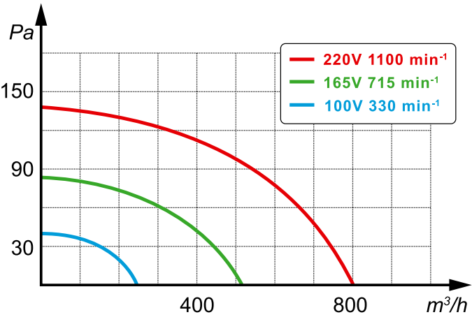
CHARACTERISTIC OF THE FAN
